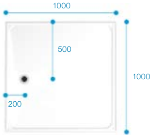
Prinia 1000x1000 shower tray illustrated above, not handed Reference Code PRIN1000x1000
