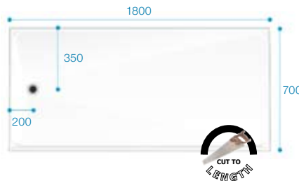
Prinia 1800x700 shower tray illustrated above, not handed Reference Code PRIN1800x700
