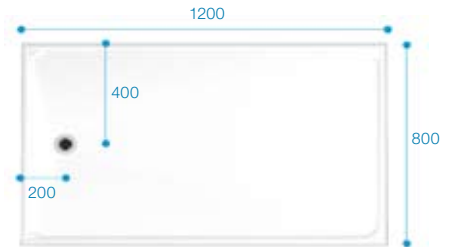
Prinia 1200x800 shower tray illustrated above, not handed Reference Code PRIN1200x800
