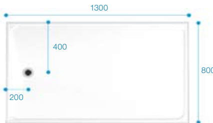
Prinia 1300x800 shower tray illustrated above, not handed Reference Code PRIN1300x800
