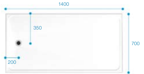
Prinia 1400x700 shower tray illustrated above, not handed Reference Code PRIN1400x700
