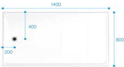
Prinia 1400x800 shower tray illustrated above, not handed Reference Code PRIN1400x800
