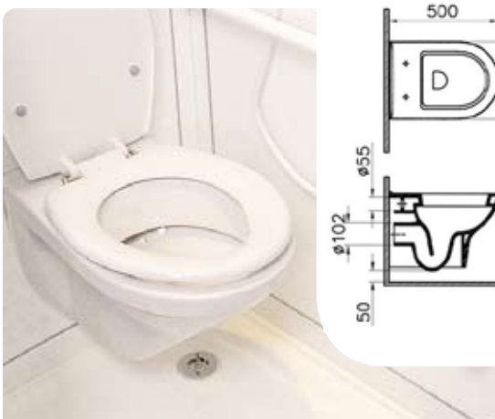
WC cubicles use a wall hung pan which allows cleaning underneath and around the WC.
